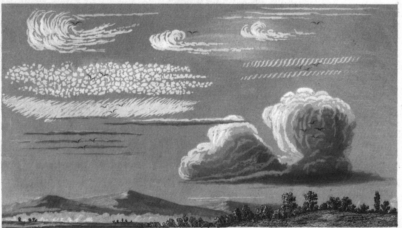
Cirrus Cirrocumulus (Cir-Cum.) Cirrostratus (Cir-Str.) various forms Cumulostratus (Cum-Str.)
